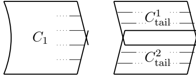
FIGURE 3. A sketch of C_1 \subset S_1 and C_{\text{tail}} \subset S_{\text{tail}} as in type (6)
