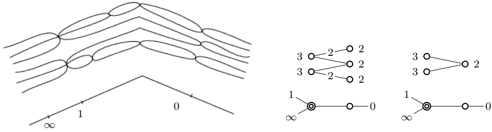
FIGURE 1. An admissible cover, and its dual graph with and without the redundant components
